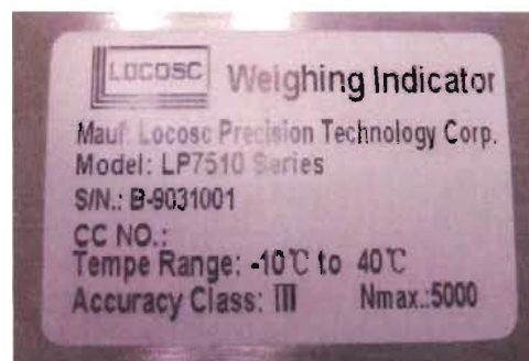
Model LP7510 – Tag with Markings
