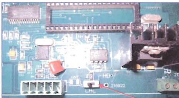
Model LP7510 – Inside View Calibration Switch
