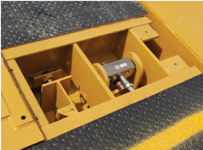
Load cell cable fully protected with conduit Bumper checking built into frame
